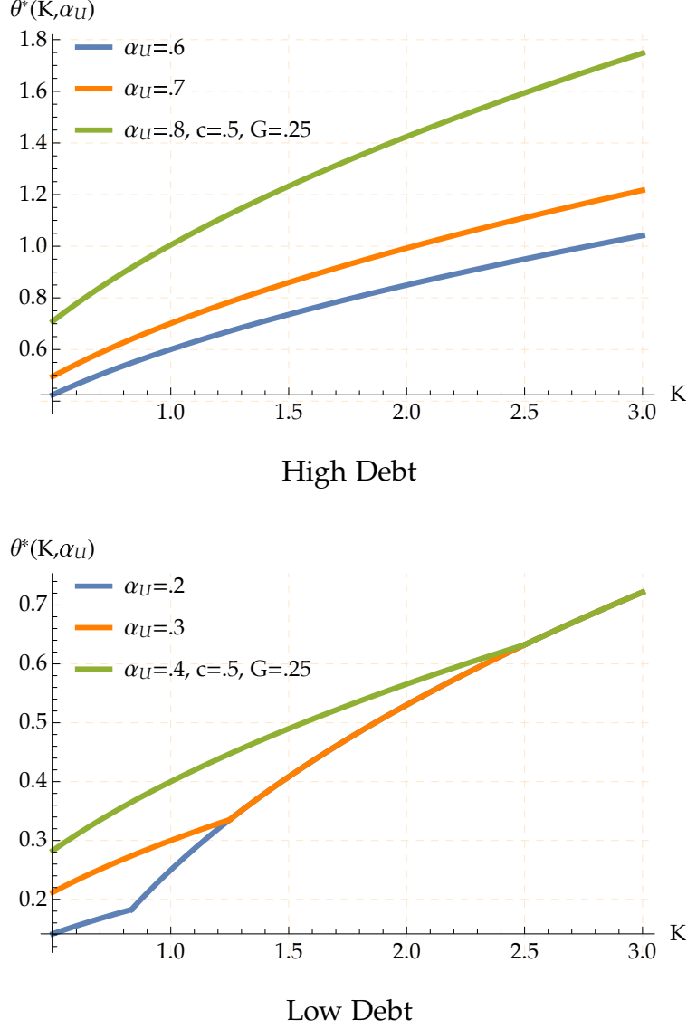
Figure 3: Illustration of Lemma 1
